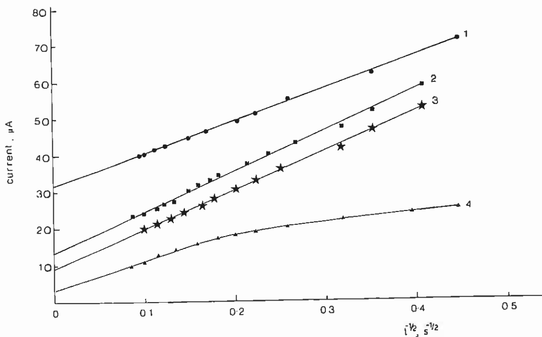
Fig. 4. Diffusion of Cu(I) through \text{Cu}_2\text{S} . Variation of current with \text{time}^{-1/2} for solutions of varying acetonitrile concentration. Key; 1, E = 0.340 V in 0.38 \text{ mol dm}^{-3} AN; 2, E = 0.400 V in 0.95 \text{ mol dm}^{-3} AN; 3, E = 0.439 V in 1.9 \text{ mol dm}^{-3} AN; 4, E = 0.509 V in 3.8 \text{ mol dm}^{-3} AN.
