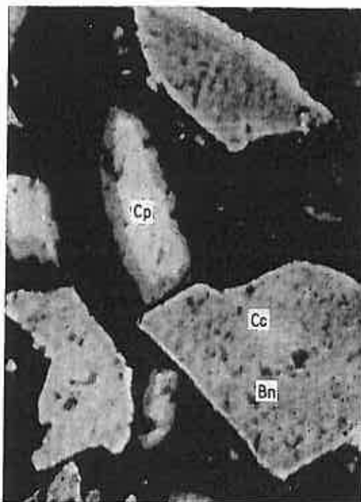
Fig. 1. Polished section of chalcopyrite crystals (X 600) after refluxing in 4 mol dm -3 AN/H 2 O containing 1 mol dm -3 Cu(I) for three hours. Bn = bornite; Cp = chalcopyrite; Cc = chalcocite.
