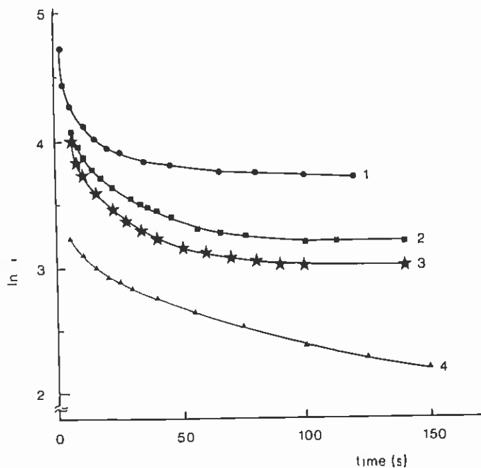
Fig. 3. Reaction of Cu(I) with chalcopryrite. Variation of current flow ( \ln i ) with time and effect of E(\text{Cu(II)/Cu(I)}) . Key, 1, E = 0.340 V in 0.38 \text{ mol dm}^{-3} AN; 2, E = 0.400 V in 0.95 \text{ mol dm}^{-3} AN; 3, E = 0.439 V in 1.9 \text{ mol dm}^{-3} AN; 4, E = 0.509 V in 3.8 \text{ mol dm}^{-3} AN.
